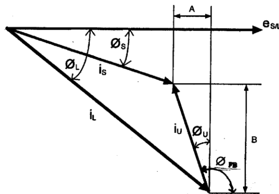
Figure 1. Phasor Diagram used to calculate the lead angle in Table 2. where,
